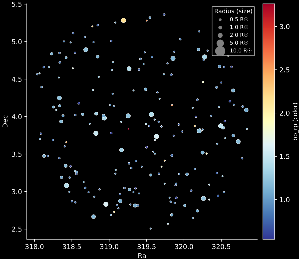
APOGEE DR17 Field: [355+56_MGA] Stars: 196
