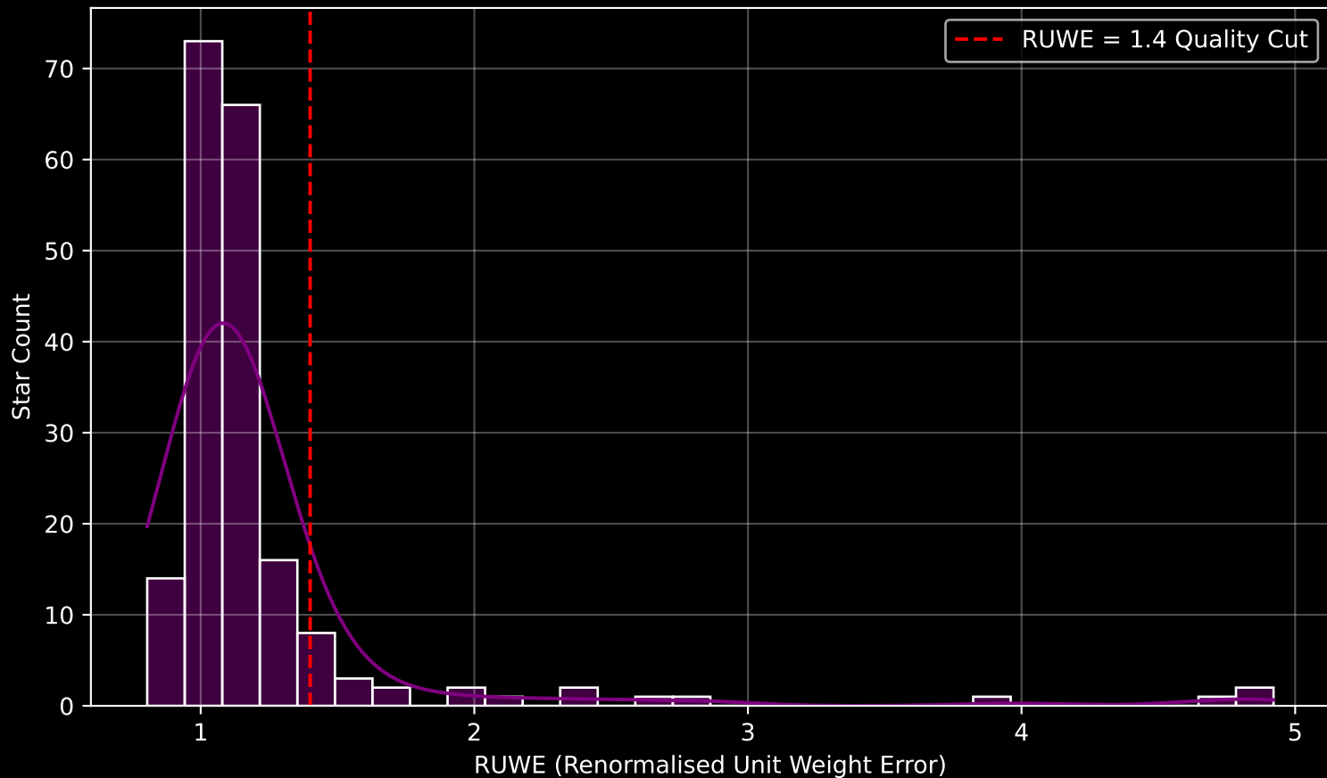
GAPOGEE DR17 Field [355+56_MGA] RUWE Distribution (n= 193)
