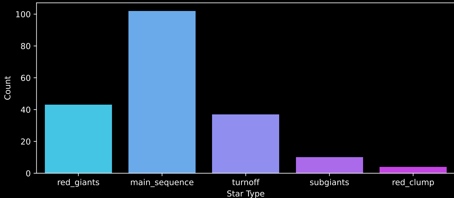
APOGEE DR17 Field: [355+56_MGA] Count plot of Star Type
