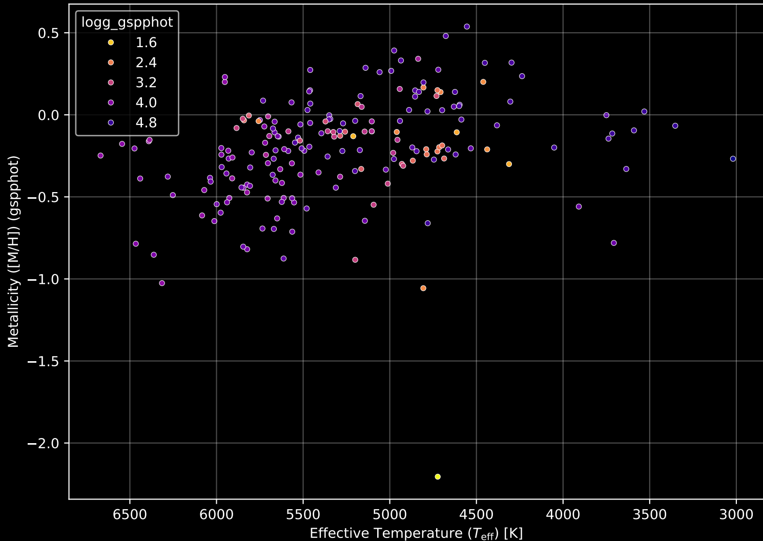
APOGEE DR17 Field: [355+56_MGA] Stellar Population Parameters (n= 196)
