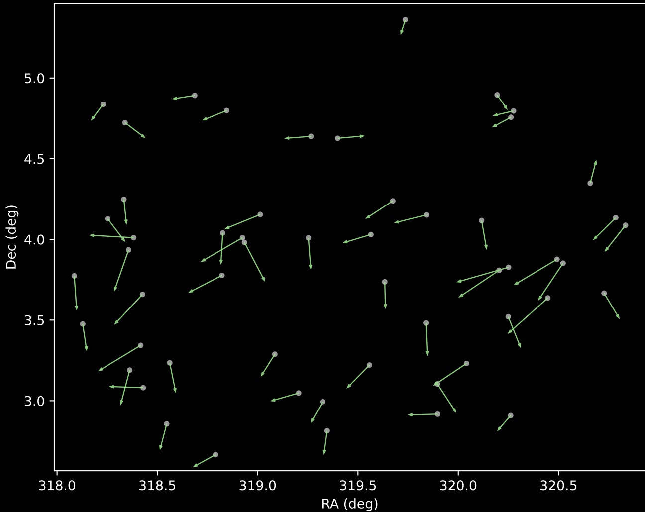
APOGEE DR17 Cluster 5 Proper Motion Vectors (n=54)
