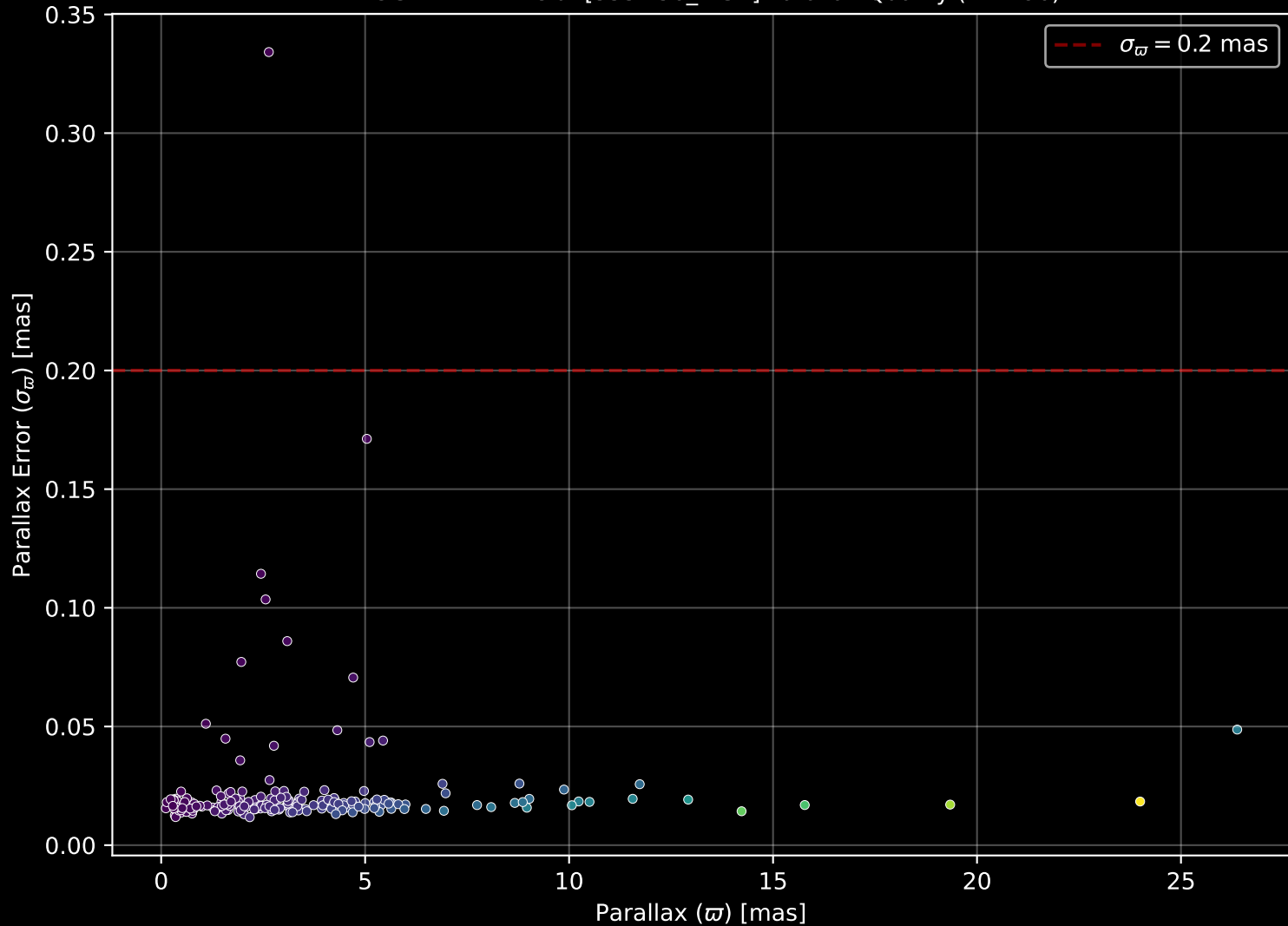
APOGEE DR17 Field: [355+56_MGA] Parallax Quality (n= 196)
