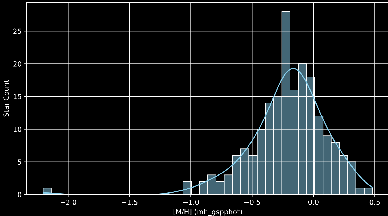
APOGEE DR17 Field: [355+56_MGA [M/H] (mh_gspphot) (n= 195)
