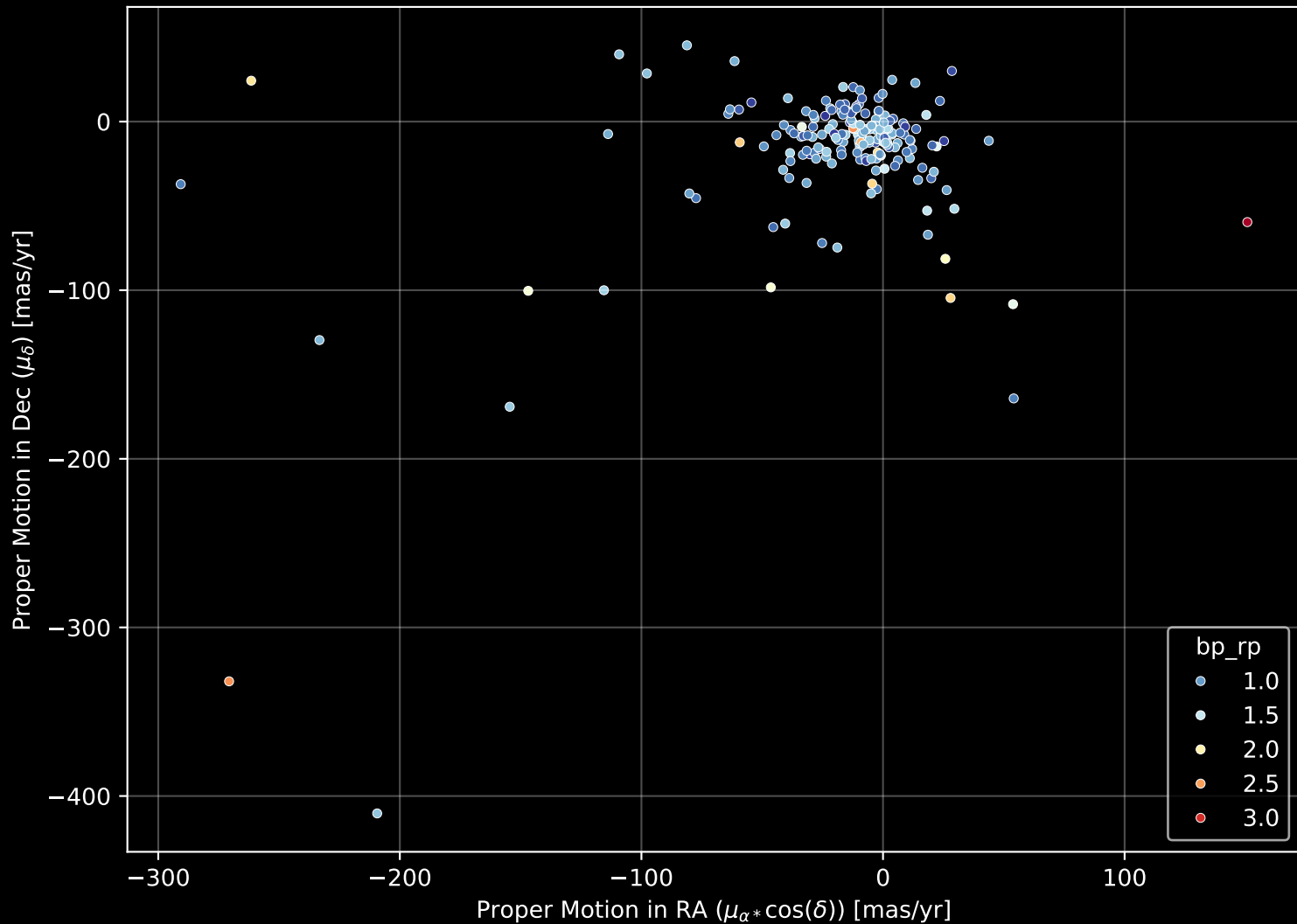
APOGEE DR17 Field: [355+56_MGA] Proper Motion Diagram (n= 196)
